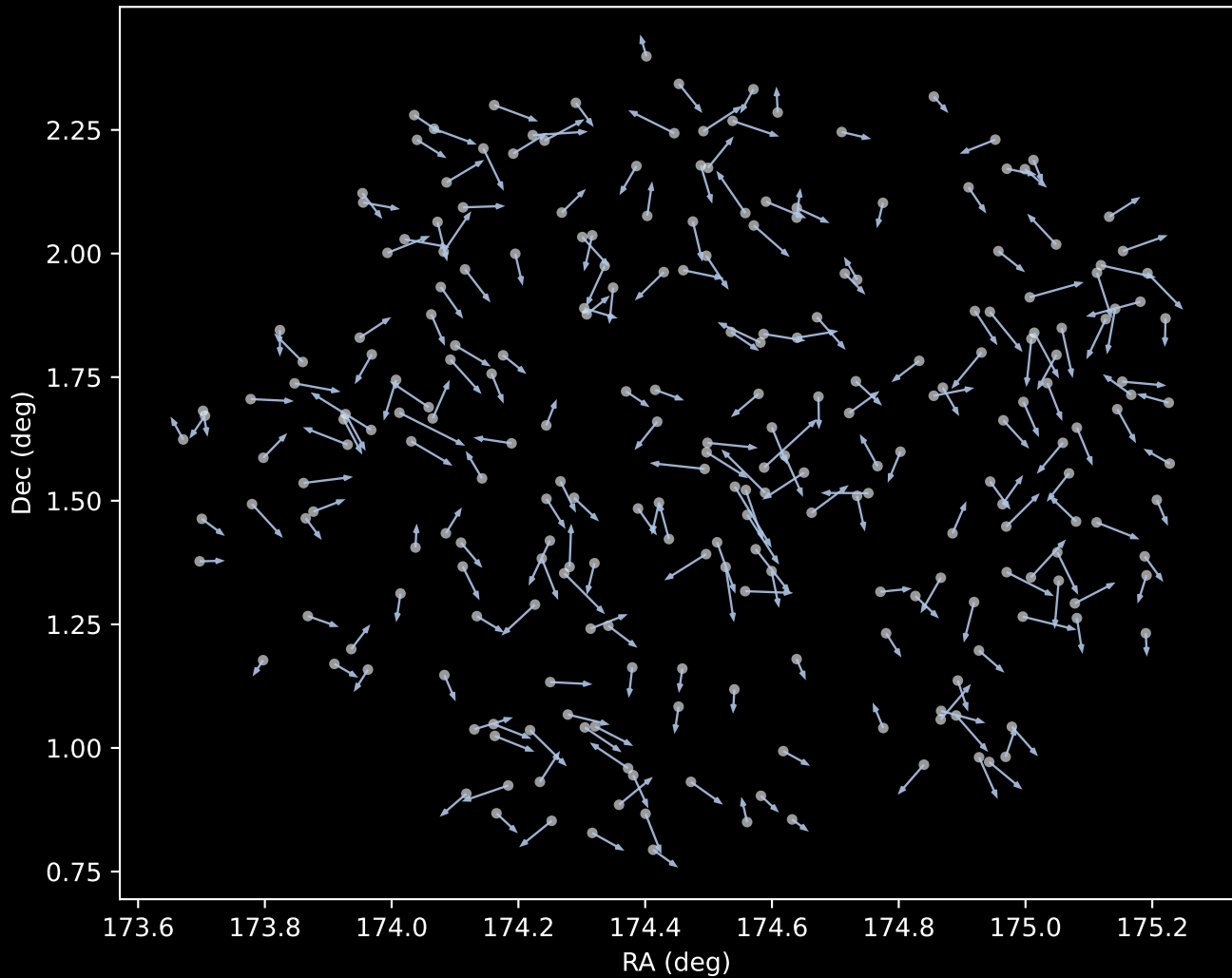
GALAH DR4 Cluster 1 Proper Motion Vectors (n=245)
