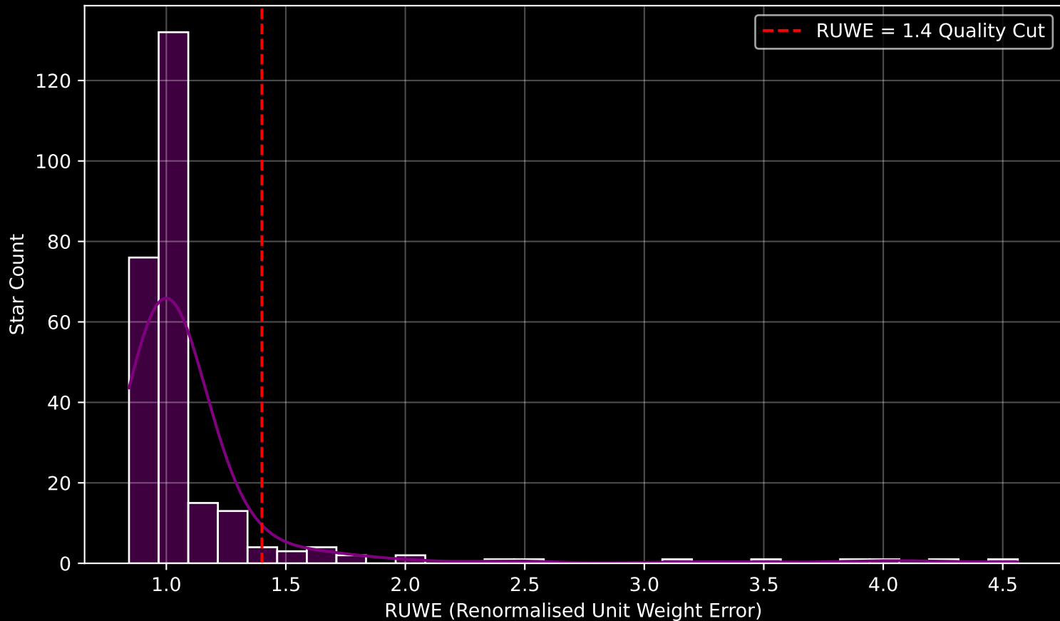
GALAH DR4 Field [1598] RUWE Distribution (n= 259)
